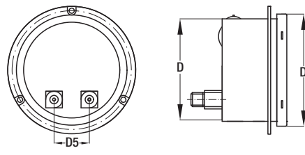
Tipo 1207: pannello, flangia anteriore attacco post. eccentrico Type 1207: Panel mounting, front flange eccentric back connection
